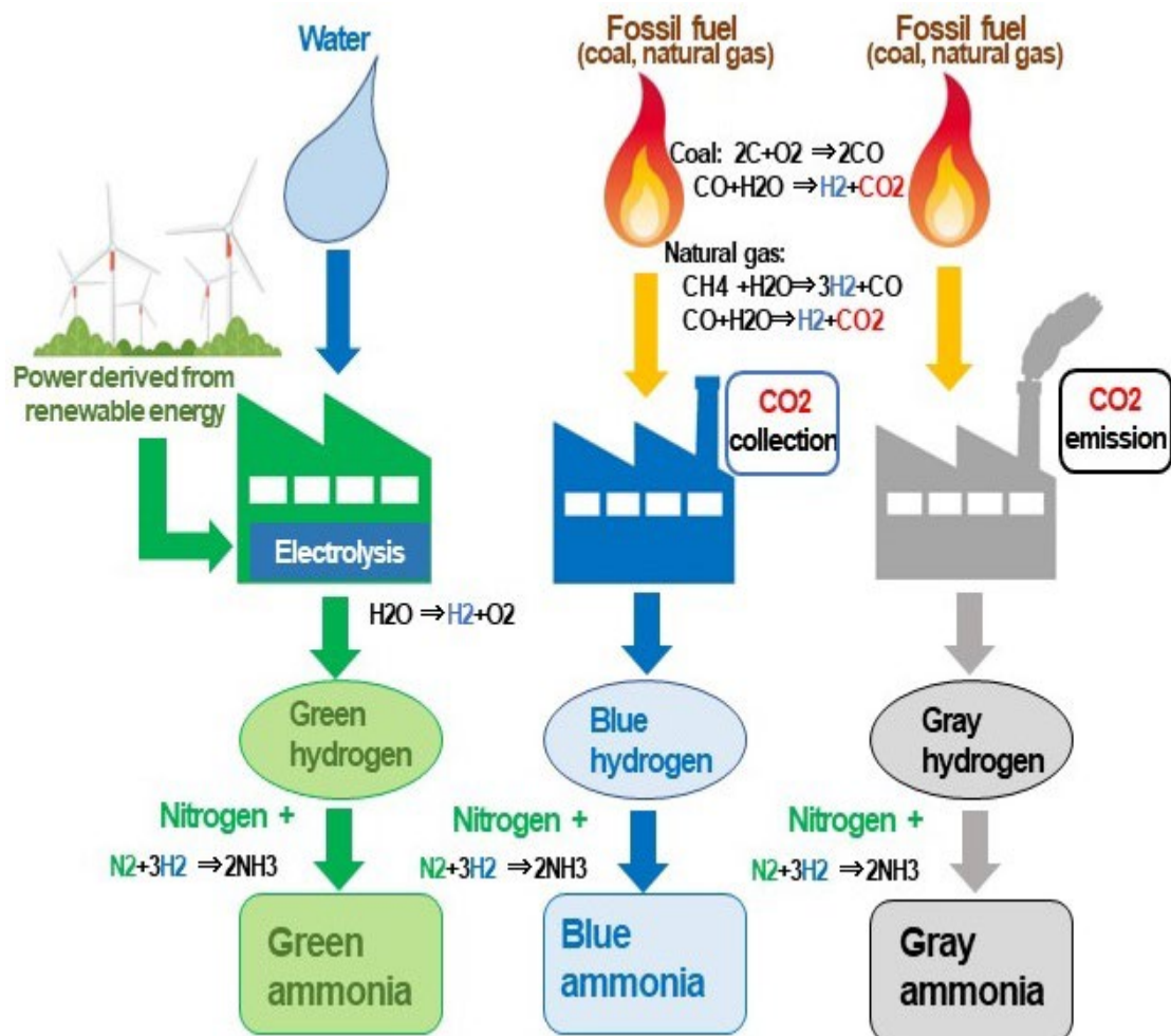
Fig. 14 Green ammonia (hydrogen), blue ammonia (hydrogen) and gray ammonia (hydrogen)
